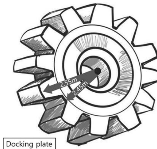
Figure 13. Shape of the gear-shape docking plate
